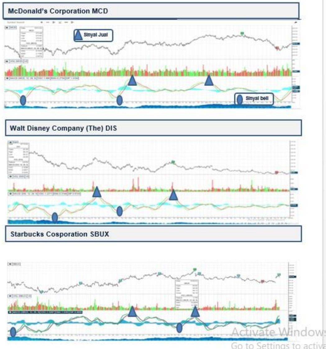
Gambar. 2 Moving Average Convergence Divergence atau MACD
