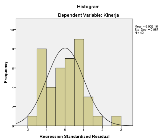
Gambar 1. Histogram
