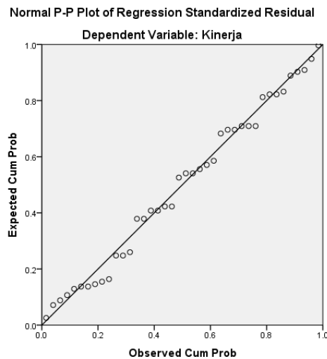
Gambar 2. PP-Plot
